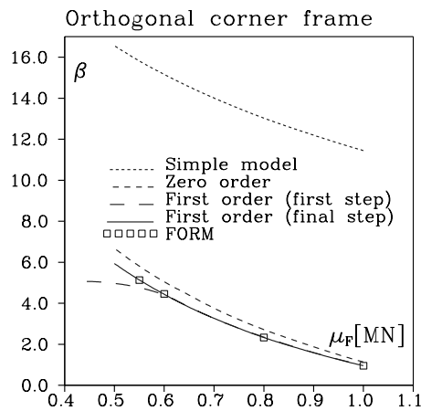
Figure 7.9: Geometric reliability index \beta as function of the mean load level \mu_F for the knee frame in Fig. 7.8.
