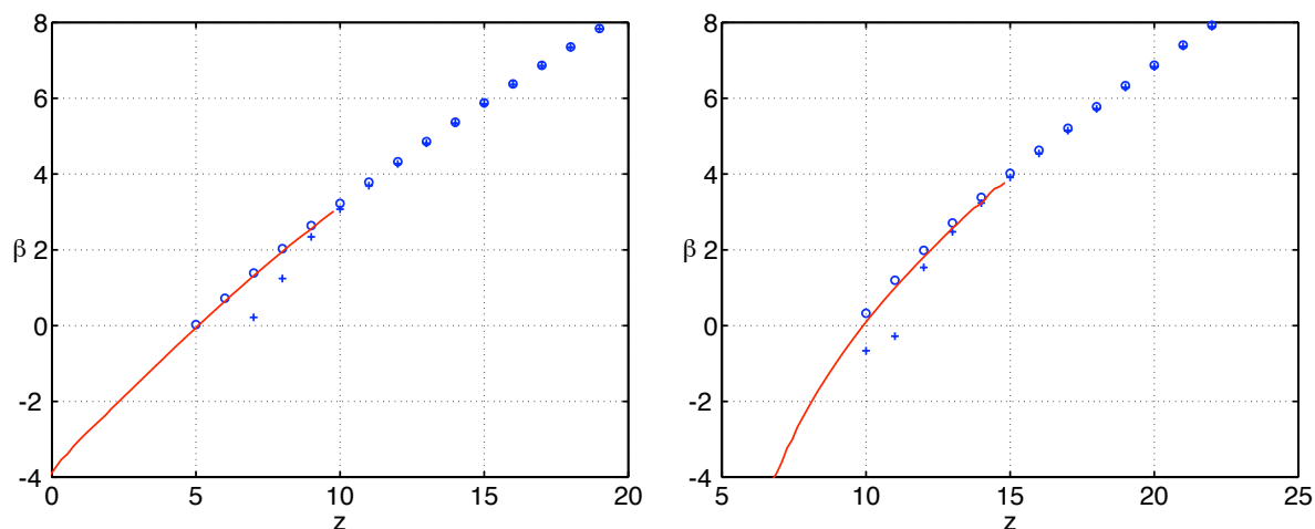
Figure 10.4: Standard Gaussian fractiles (reliability indices) \beta = \Phi^{-1}[P(\max\{Z_1, \dots, Z_N\} \leq z)] determined by simulation (solid curve, sample size 100 000), FORM by RF algorithm \circ , and after curvature correction + . The hierarchical system has 5 levels ( n = 4 ) with 4 variables at each level. All random variables are either standard Gaussian: f(x) = \exp(-x^2/2)/\sqrt{2\pi} (left), or standard Rayleigh: f(x) = x \exp(-x^2/2), x \geq 0 , (right). The second order corrections are insignificant.
