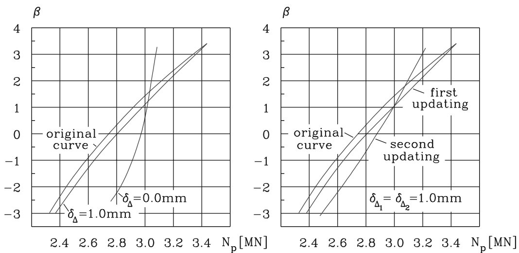
Figure 13.5: Distribution functions before and after updating with respect to the prestressing force N(10.000 \text{ days}) for the concrete beam with cross-section as in Fig. 13.4 and with span 10 m and bending moment 1 MNm. (The ordinate axis scale is the fractile scale for the standardized normal distribution, and \delta_\Delta = D[\Delta] .)
