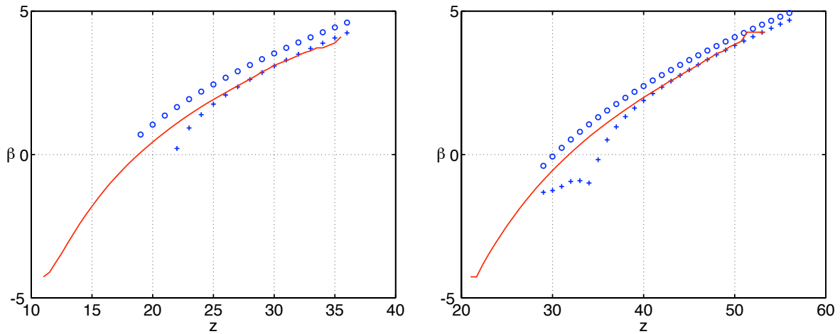
Figure 10.6: Caption as in Fig. 10.4 except that all random variables of the hierarchical system are gamma distributed: f(x) = x^{k-1} e^{-x} / \Gamma(k), x \geq 0 , here standard Erlang distributions of mean k = 2 (left) and k = 4 (right). The second order corrections are substantial.
