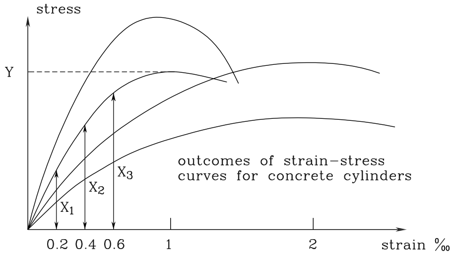
Figure 4.4: Forecasting of concrete stress-strain curves on the basis of measured values for small strains.
